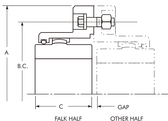
Shrouded Bolt — Falk G10 (1000 Series) Half &amp; Other Half
