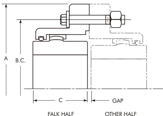
Exposed Bolt — Falk G20 (1000 Series) Half &amp; Other Half
