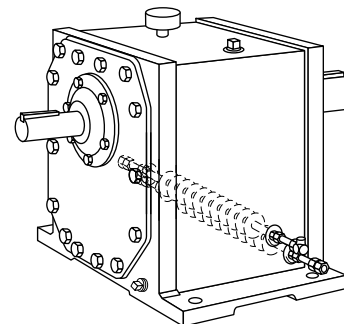
Cooling Tubes
